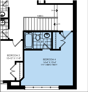
OPT. SECOND FLOOR BEDROOM 4 AND ENSUITE
